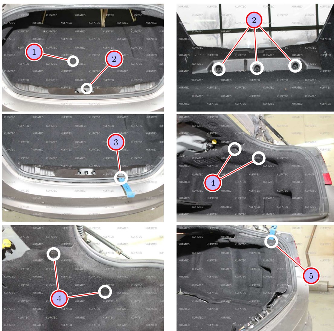
Figure 4: Removing trunk trim panel
