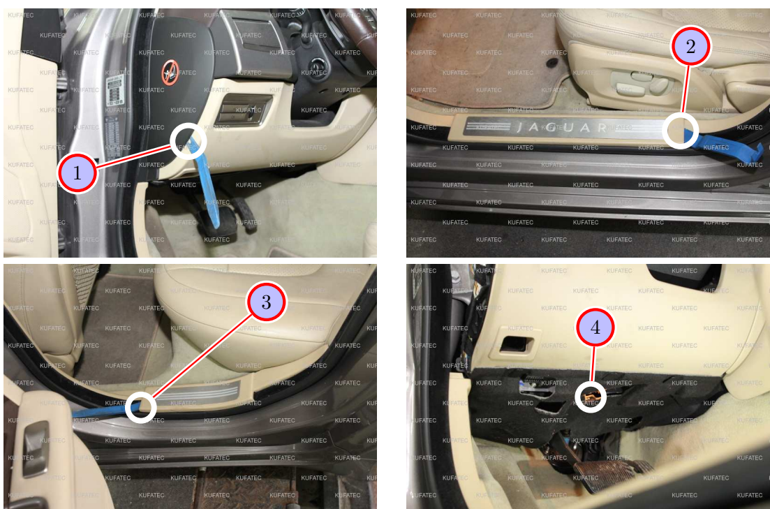
Figure 9: Removing trim panels
