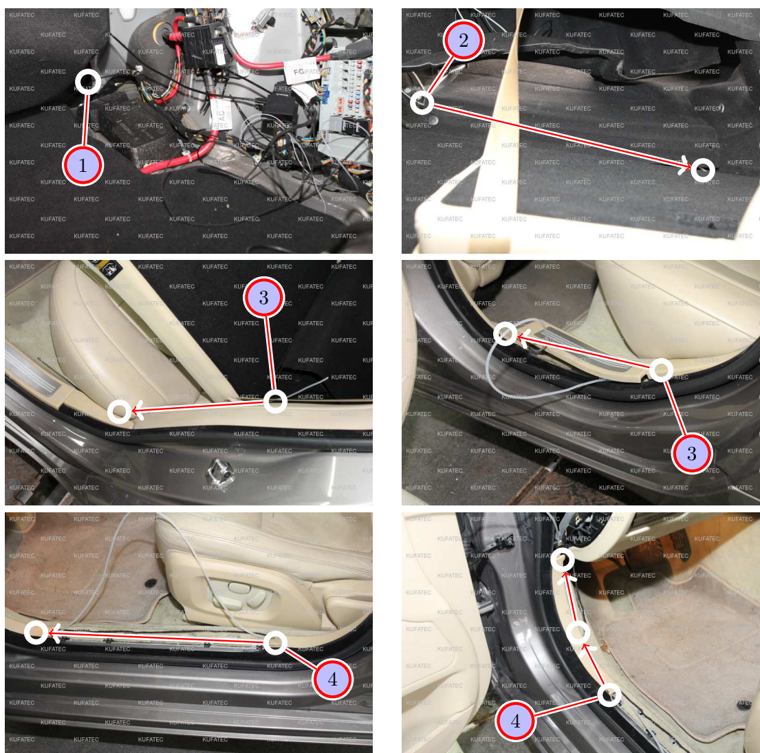
Figure 10: Pushbutton cable routing
