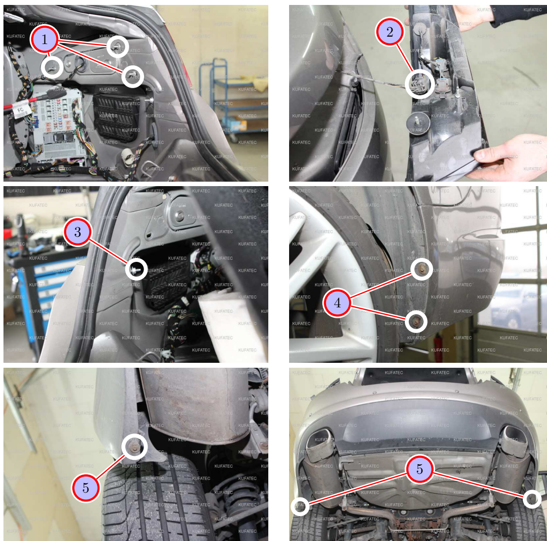
Figure 6: Removing taillights and bumper
